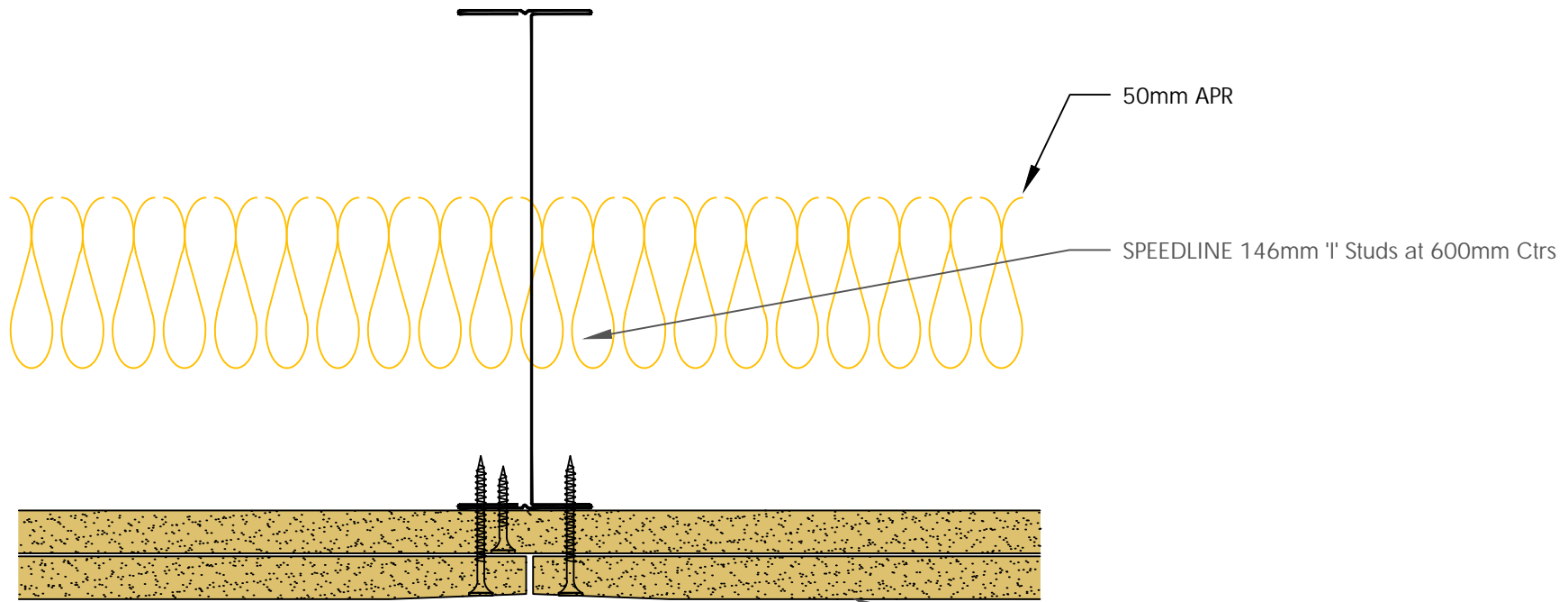
50mm APR SPEEDLINE 146mm 'I' Studs at 600mm Ctrs 2x12.5mm Siniat GTEC Standard Board fixed with SPEEDLINE Drywall Screws at 300mm centres (200mm centres at external angles). Ref to table for fixing length.
